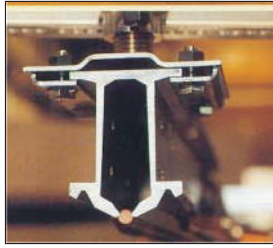
Conductor Rail Profile shown with contact wire
