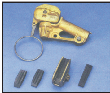
TROLLEY SHOE CARBON
