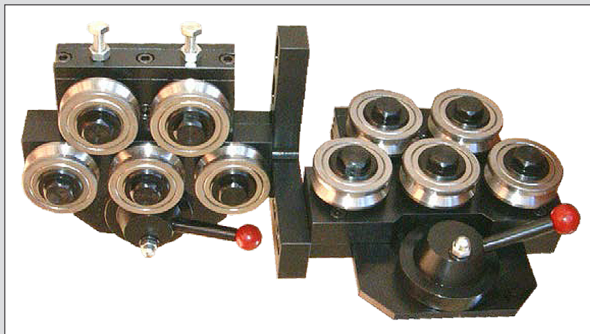
Two Straighteners combined to straighten in 2 planes
